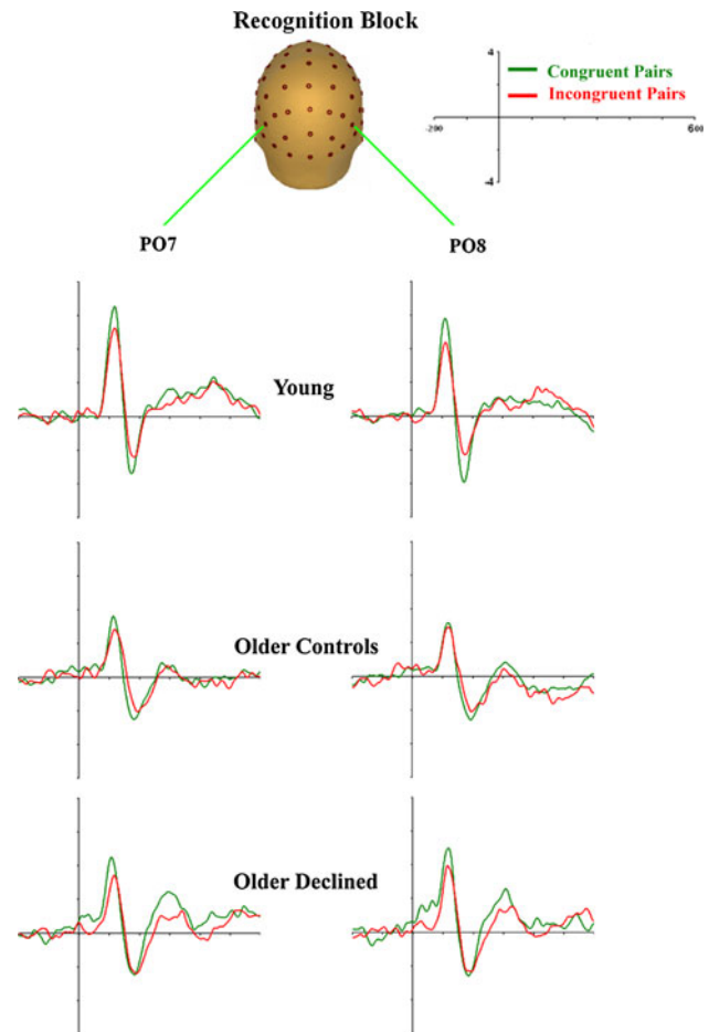
Fig. 6 Recognition block: P100 and P300 for congruent and non-congruent pairs for young, older controls and older declined adults
