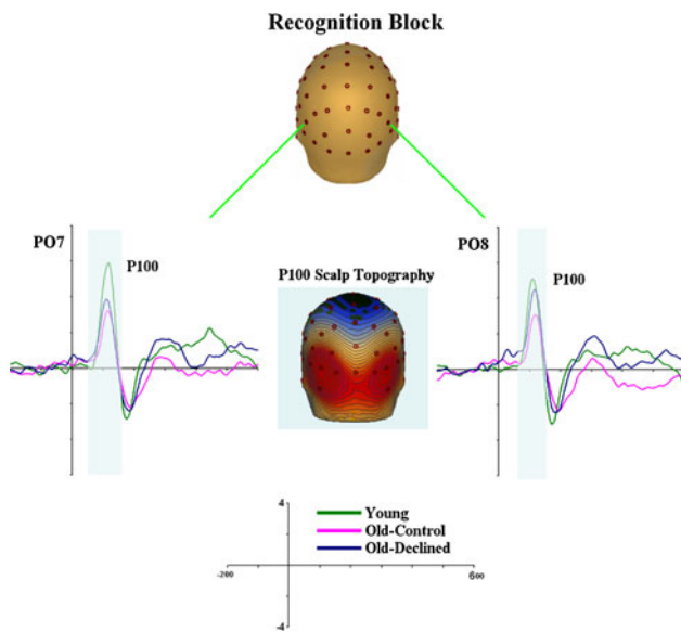
Fig. 5 Recognition block: P100 head maps and ERPs of significant electrodes PO7 & PO8
